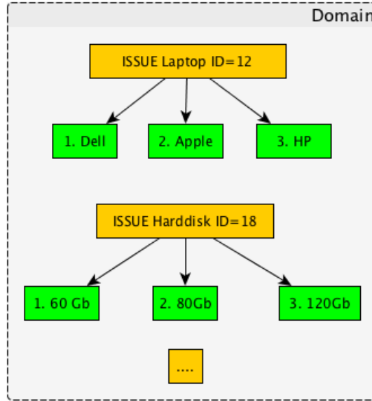
Figure 1: An example domain for laptop negotiation. Issues are orange, values are green
