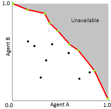
Figure 3: A point indicates the utility for both parties of a bid. The red line is the Pareto optimal frontier.
