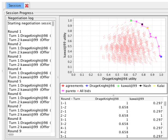
Figure 10: Bilateral progress panel.
